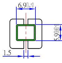
SECTION G-G
